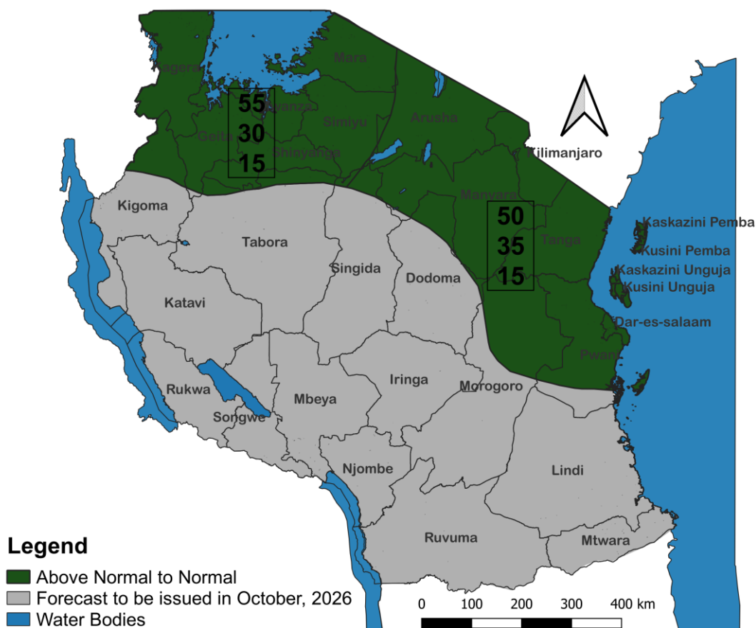
Figure 1: Outlook for October to December, 2026 rainfall season.
