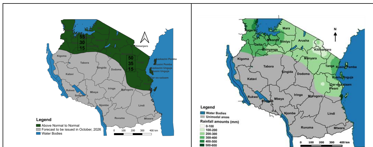
Figure 2: Left: Rainfall Outlook for Vuli (October – December) 2026 season and right: Long-term average (30 years) of October to December climatological rainfall (1991-2020).
